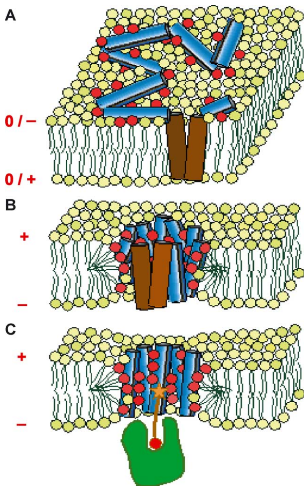
Fig. 2. Transition from closed pore (surface-bound flexible helical array) to open state of colicins may involve transient or permanent local formation of toroidal lipid-lined pores. (A) Closed state of pore after colicin binding to membrane or after pore-closing in the presence of a trans-positive potential. (B) Toroidal configuration of the open pore state. (C) Cross section of toroidal pore with an example of Cys (brown star) labeled through a 10–15-Å linker with biotin (red circle), and bound avidin (green). Helices in front of channel, shown in (B), are removed for visualization of pore interior. Anionic lipids that interact with basic side chains in the pore lining of the toroidal pore structure are shown in red.
