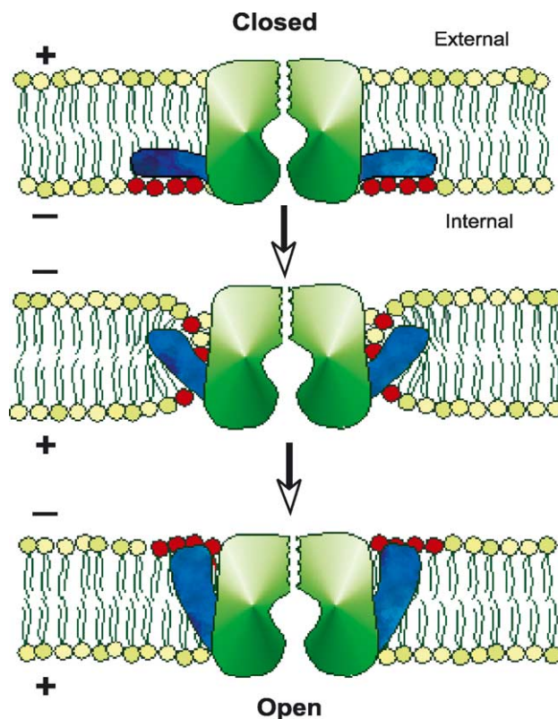
Fig. 5. Voltage-gating of K^+ channel may involve transient formation of local non-bilayer lipid structures around a translocated voltage-sensing segment (blue) to decrease the energetic cost of insertion of the gating charge (Arg) into the bilayer.
