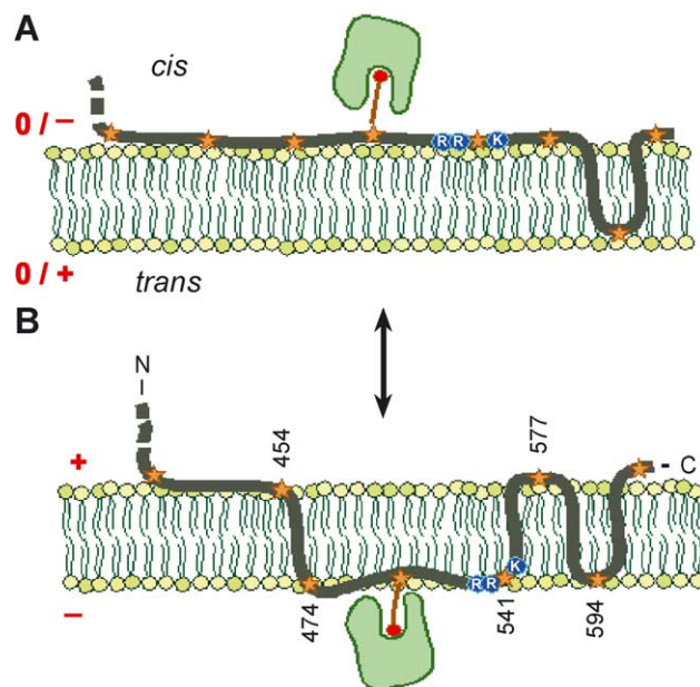
Fig. 4. Detection of voltage-dependent translocation of a large part of the pore-forming domain of colicin Ia to the trans -side of the membrane, using biotin–streptavidin complex formation. Gating changes carried by Arg534, Arg537, Lys544 are blue [1].
