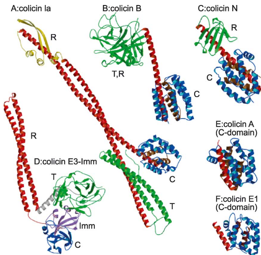
Fig. 1. Ribbon diagrams of the X-ray structure of colicin Ia (A), B (B), N (C) and E3 (D), and pore-forming domains of colicins A (E) and E1 (F). Pore-forming (cytotoxicity) domains are shown in blue and brown (hydrophobic hairpin); connecting single helix (B, C, E, F) or double-helix colicin E3 coiled-coil (A, D), red; translocation domain, green; immunity protein in colicin E3 (D), magenta.
