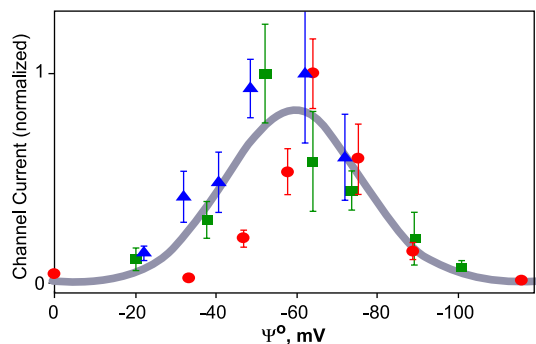
Fig. 3. Macroscopic steady-state current in planar bilayers as a function of surface potential, calculated from Gouy-Chapman theory. Data were normalized relative to the amplitude of the maximum current for different ionic strengths; i.e., at 25, 30, and 70 mol% DOPG for 0.1 (circles, red), 0.3 (squares, green), and 1.0 M (triangles, blue) KCl, respectively.
